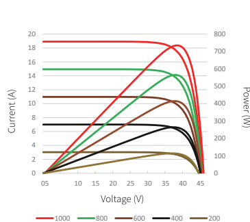
Current-Voltage & Power-Voltage Curves (720W)
